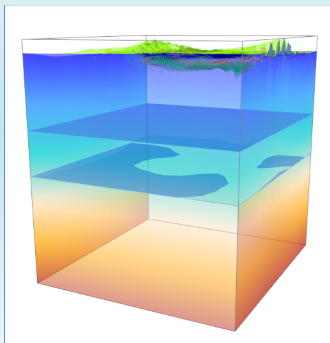
Figure 1: 3D Underworld model of Latrobe Valley geothermal properties, visualised using gLucifer (to view and rotate interactively in 3D, open in Acrobat Reader v. 8.0 or higher).
