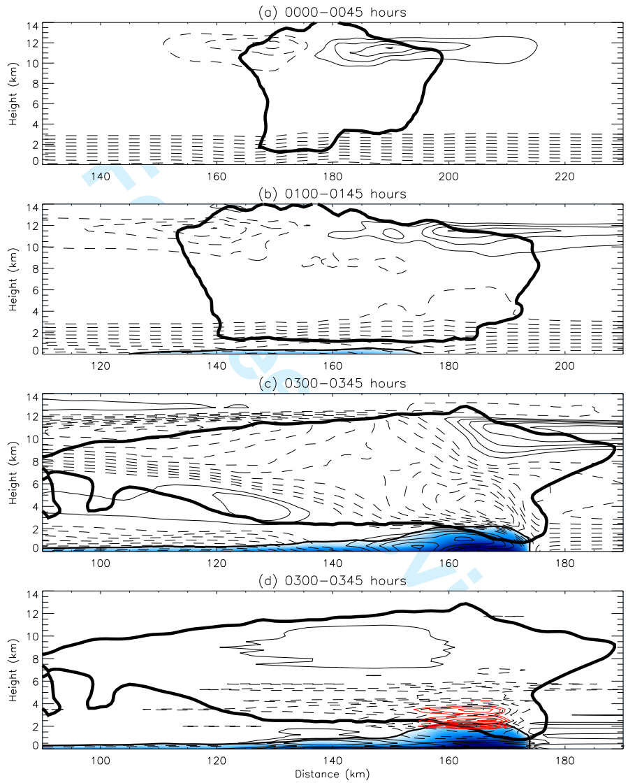
Figure 2. Cross-section of cloud (cloud mixing ratio contour outline 0.1 g kg -1 is shown by solid black line) averaged in the y-direction and time-averaged over the following time periods: (a) 0000-0045 hours, (b) 0100-0145 hours and (c) & (d) 0300-0345 hours when the system is fully developed. (a)-(c) shows contours of u (every 2.0 m s -1 , with zero removed) - positive values shown by solid lines and negative by dashed) for medium 1 km resolution cyclic domain. The cold pool is shown by blue shading, using an outer contour of -1°C temperature perturbation. (d) The black contours are pressure perturbations every 30 Pa, with negative values shown by dashed lines and positive values shown by solid lines. The red contours shows the pressure perturbations every 30 Pa, less than 150 Pa i.e. the region of lowest pressure.
