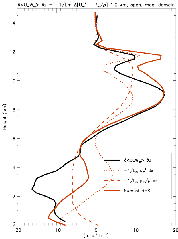
Figure 15. Terms in the relationship \frac{\partial}{\partial z} \langle u_m w_m \rangle = -\frac{1}{L_m} \Delta \left[ u_m^2 + \frac{p_m}{\rho} \right]_0^{L_m} for the open lateral boundary conditions for medium domain. Averaged over 0400–0500 hours during the mature stage of evolution. Sum of the terms on the RHS are shown by the solid red line.
