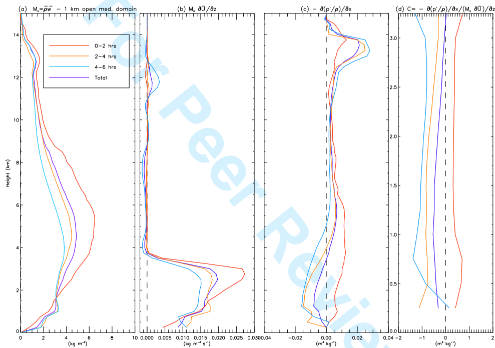
Figure 13. Terms in the relation used in the Gregory parametrisation scheme, -\frac{\partial}{\partial x} \left( \frac{p}{\rho} \right) \propto C_u M_u \frac{\partial \overline{U}}{\partial z} - shows (a) M_u = \overline{\rho w} , (b) M_u \frac{\partial \overline{U}}{\partial z} , (c) -\frac{\partial}{\partial x} \frac{p'}{\rho} \Big|_u and (d) C_u where C_u = \frac{-\frac{\partial}{\partial x} \frac{p'}{\rho}}{M_u \frac{\partial \overline{U}}{\partial z}} but only up to 3.25 km - (the height of the shear level) for the 1 km resolution medium open domain. These terms are averaged across time periods and across updrafts ( > 1 \text{ m s}^{-1} ) for each height level.
